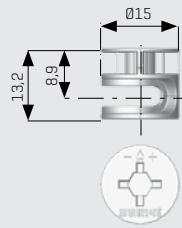
Cam 13.2 mm
