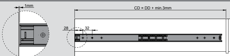
Drawer Dimensions
