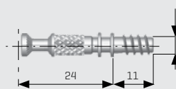
24 mm Steel Bolt Euro Screw Type
