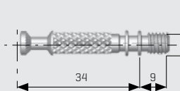
34 mm Steel Bolt M6 Screw Type
