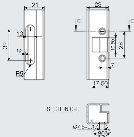
Hinge Cup Dimensions
