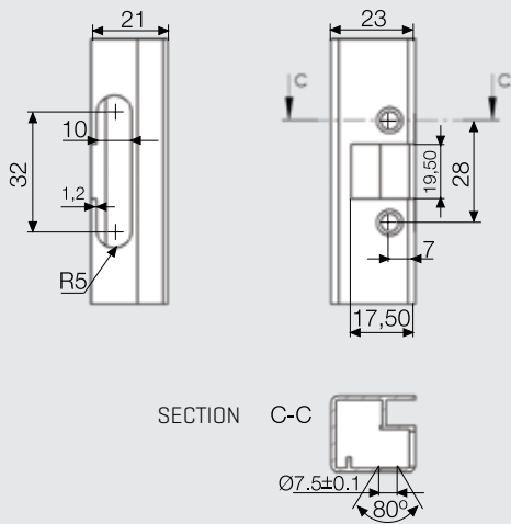
Hinge Cup Dimensions
