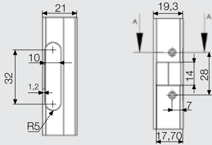
Hinge Cup Dimensions
