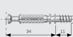
34 mm Steel Bolt Euro Screw Type
