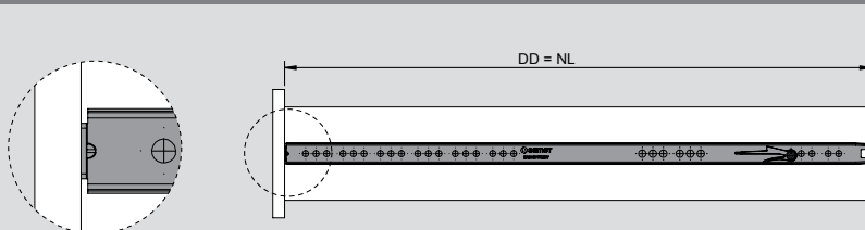
Drawer Dimensions
