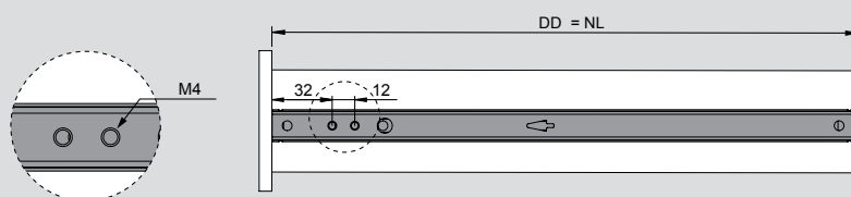
Drawer Dimensions
