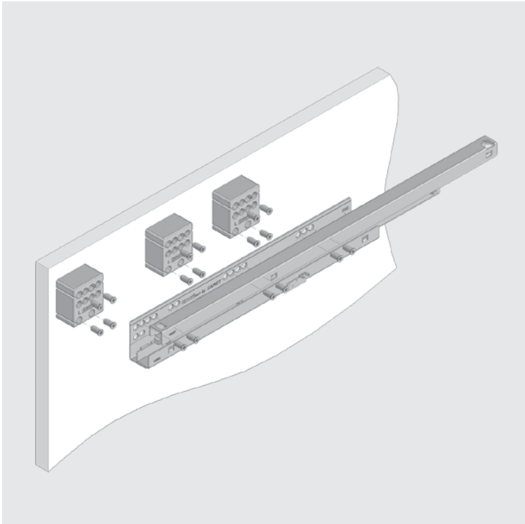
Slide Screw Location
