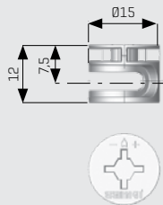
Cam 12 mm
