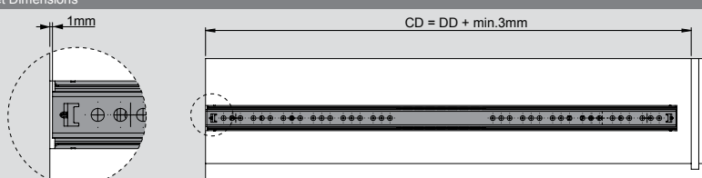
Drawer Dimensions
