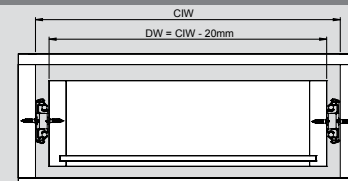
Technical Dimensions
